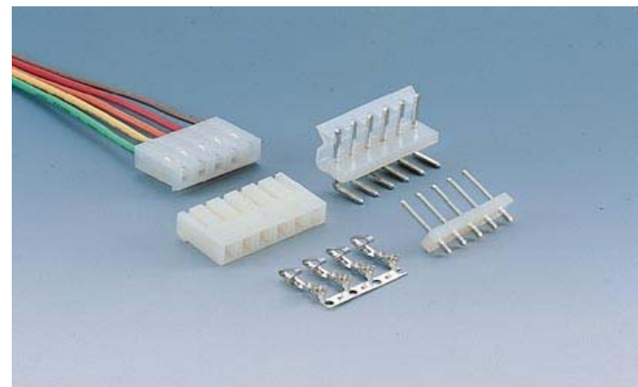
3.96mm(.156") Housing/Wafer/Header
