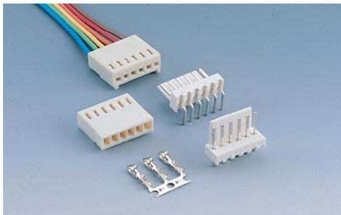
2.54mm(.100") Housing/Wafer
